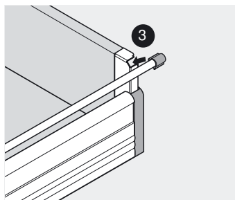
Bakre montering
