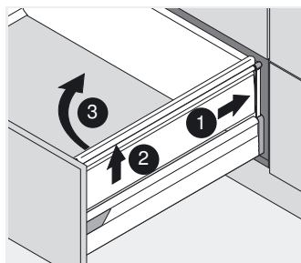
Demontering
