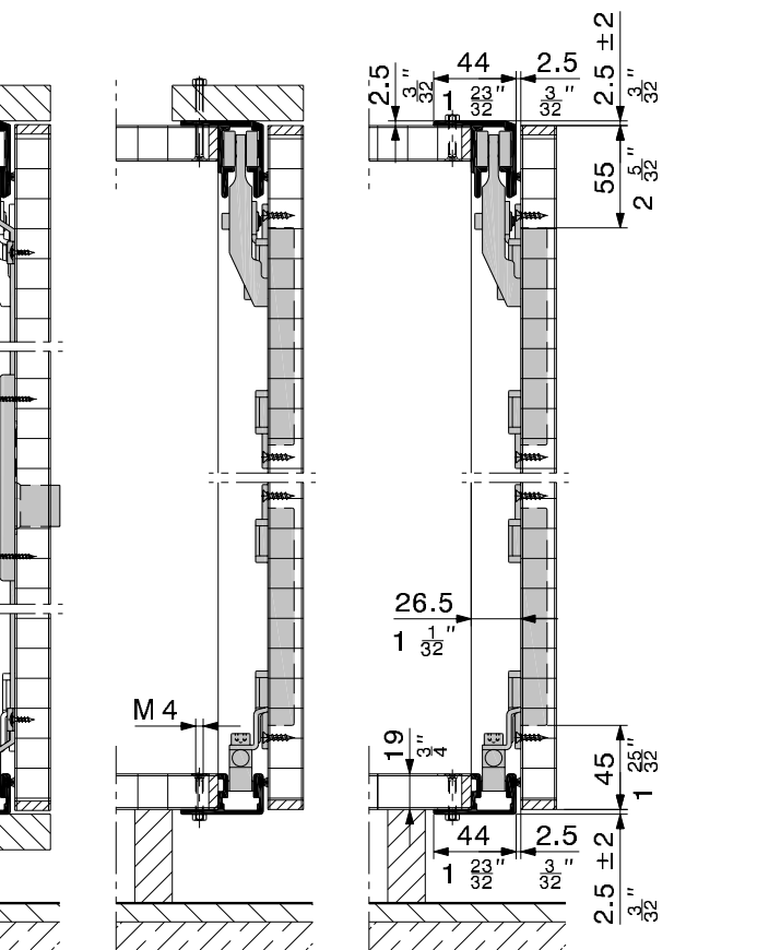
Inlaying doors Semi-overlaying doors Overlaying doors
