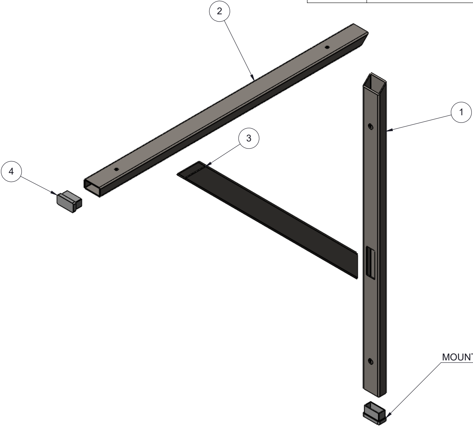
EXPLODED VIEW
