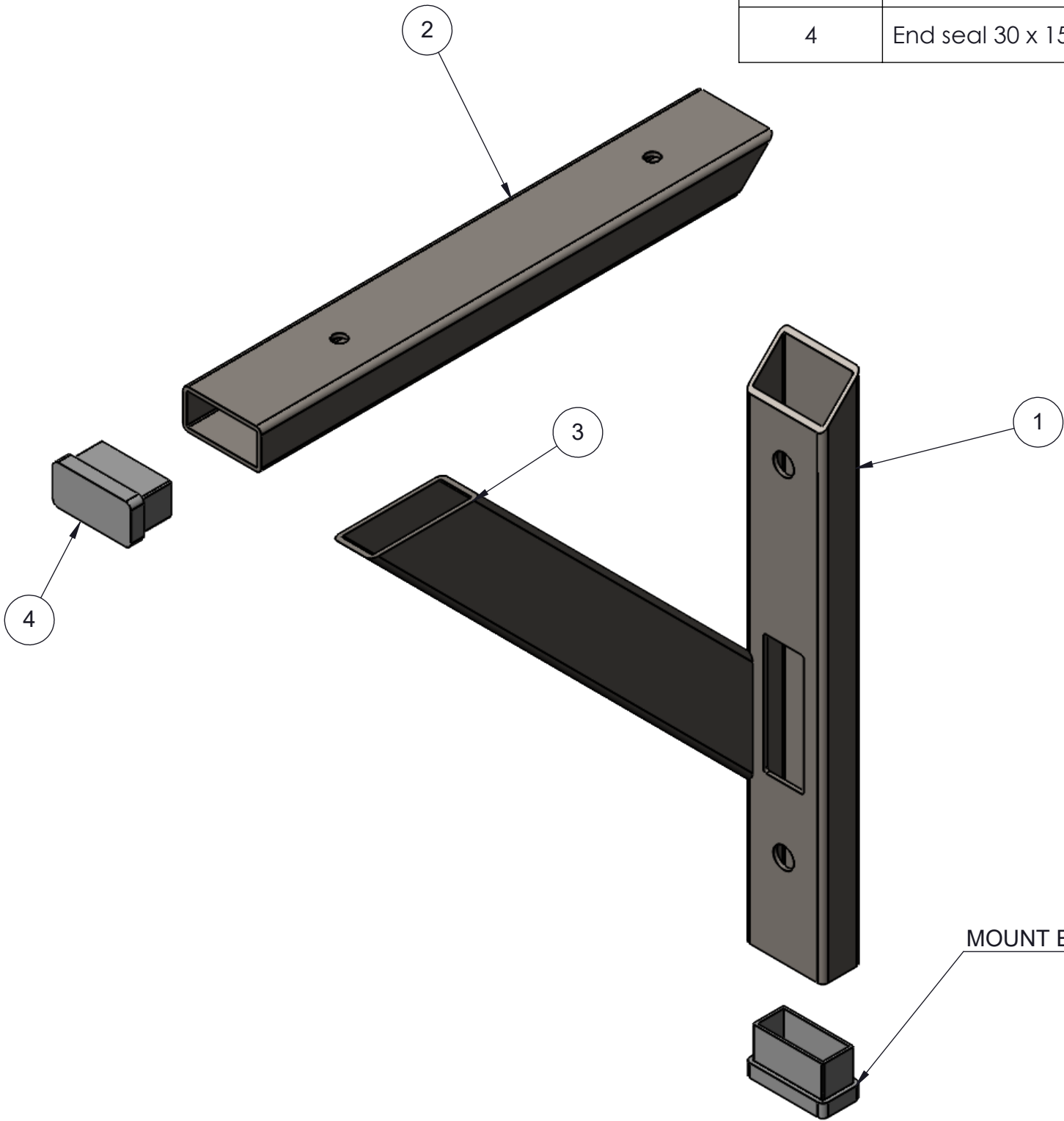
EXPLODED VIEW
