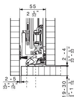
Connector 55 mm ( 2\frac{3}{16} " ) Maximum door thickness: 30 mm ( 1\frac{3}{16} " )
