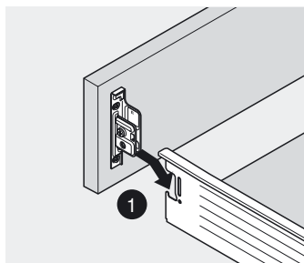
ZSF.1700/1800 Montering
